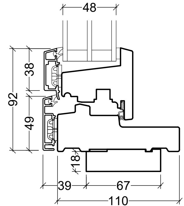
Cill packer type 18x67 Check reveal packer type 18x67
